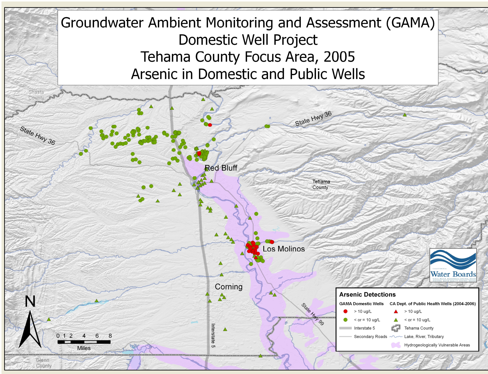
Figure 4: Arsenic Concentrations
