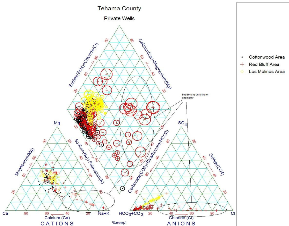
Figure 6: Piper Diagram of Groundwater Geochemical Composition
